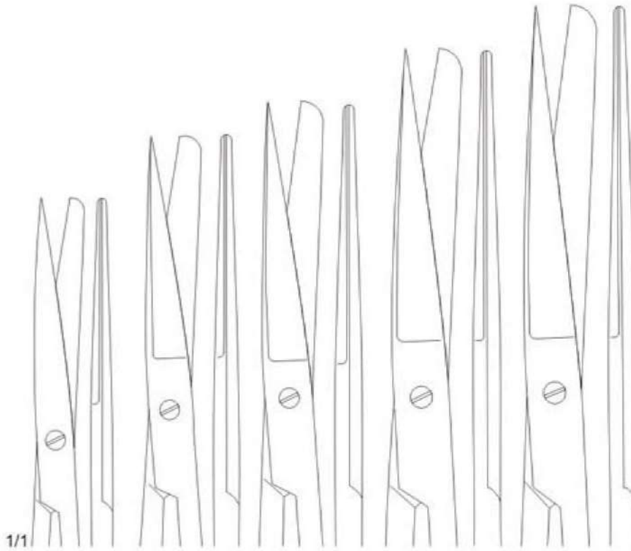
1/1 02-059-11 11.5 cm / 4½" 02-059-13 13.0 cm / 5" 02-059-14 14.5 cm / 5½" 02-059-16 16.5 cm / 6½" 02-059-18 18 cm / 7½"
